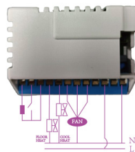
Connection 3: 2-pine ON/OFF +floor heating
