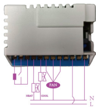
Connection 2: 4-pine ON/OFF +3 speed fan
