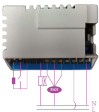
Connection 1: 2-pine ON/OFF +3 speed fan
